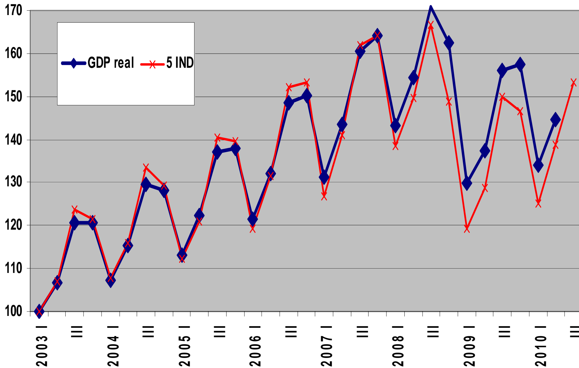
Indices of real GDP and of the volume of output in 5 industries (1st quarter of 2003 = 100%)
