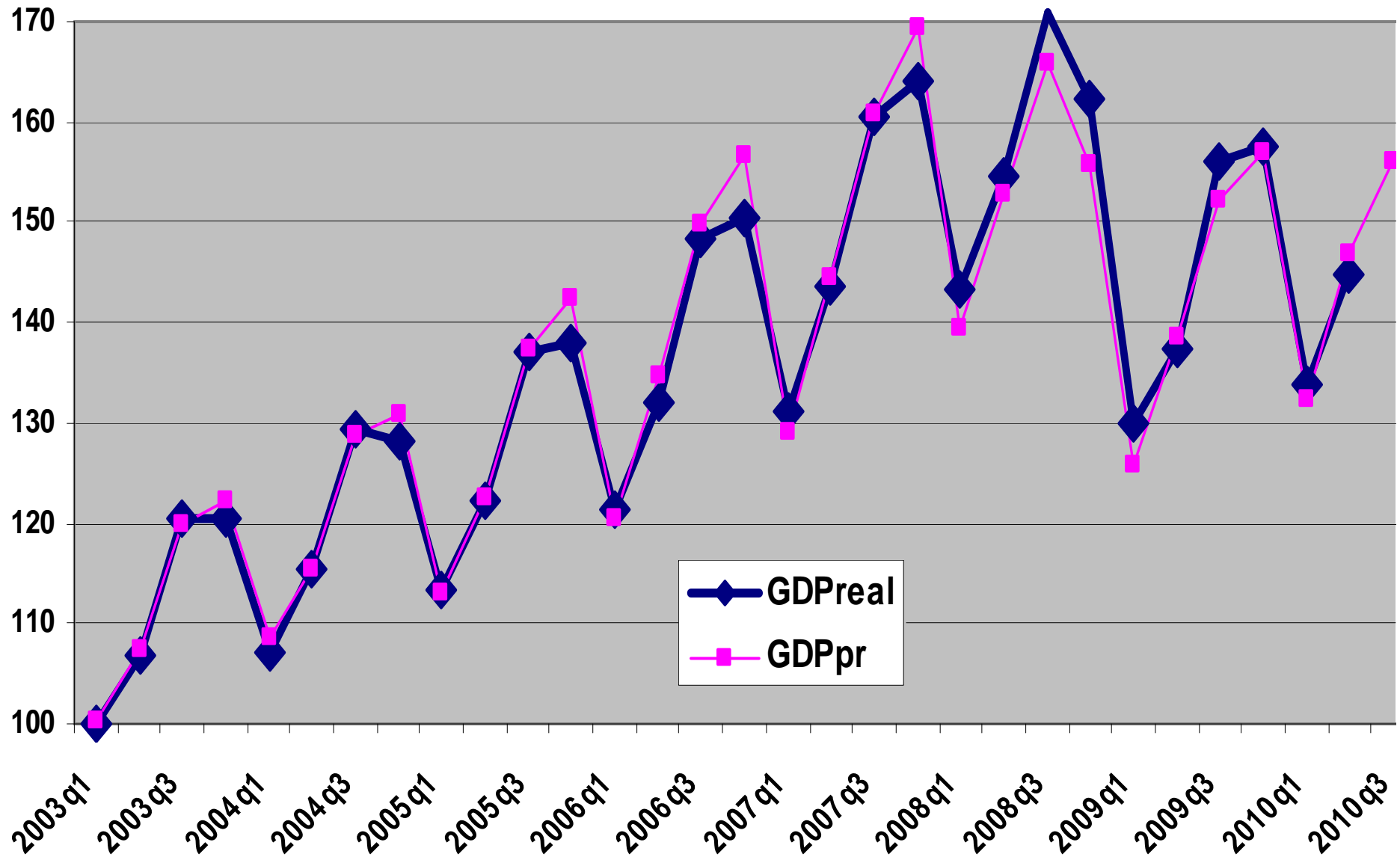
Predicted and actual real GDP, Q1/2003=100% (prediction is based on volume of output in 5 industries and real incomes)
